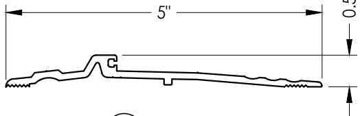
40 THRESHOLD
