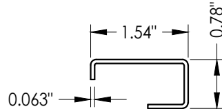
86 GLASS STOP
