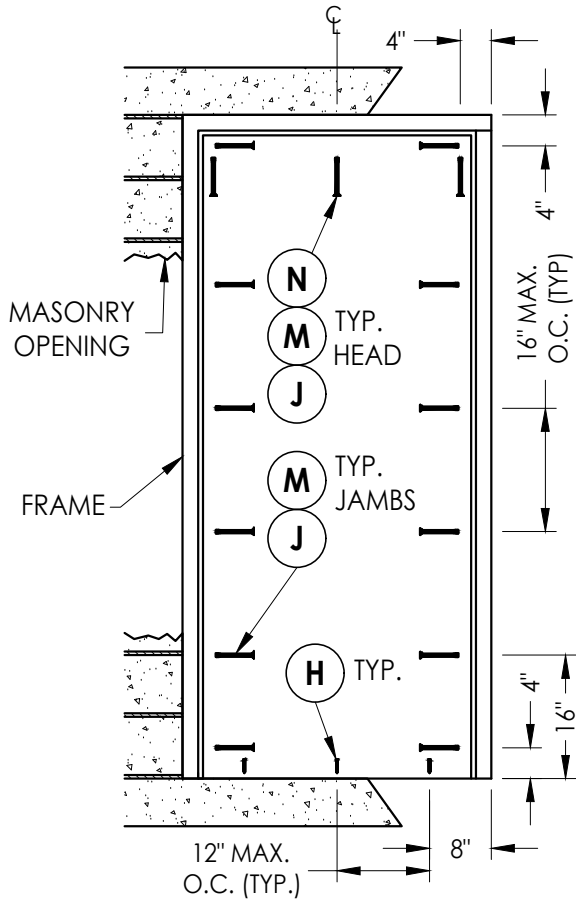
FRAME ANCHORING
